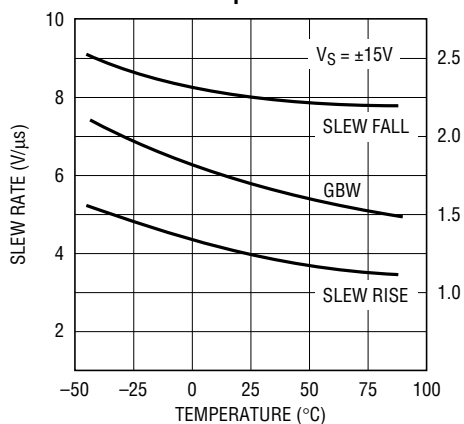
Slew Rate, Gain-Bandwidth Product vs Temperature
