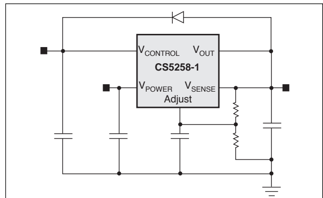
Figure 3: Diode protection against V CONTROL short circuit conditions.
