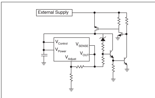
Figure 2: Example clamp circuitry for V POWER - V OUT > 6V.
