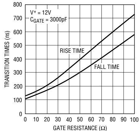
Transition Times vs R_{Gate}
