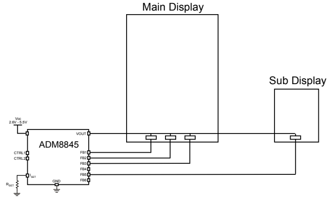
Figure 30. ADM8845 Driving three Main and one Sub
