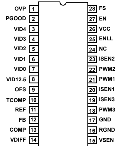
ISL6565ACB (SOIC), ISL6565ACV (TSSOP) TOP VIEW
