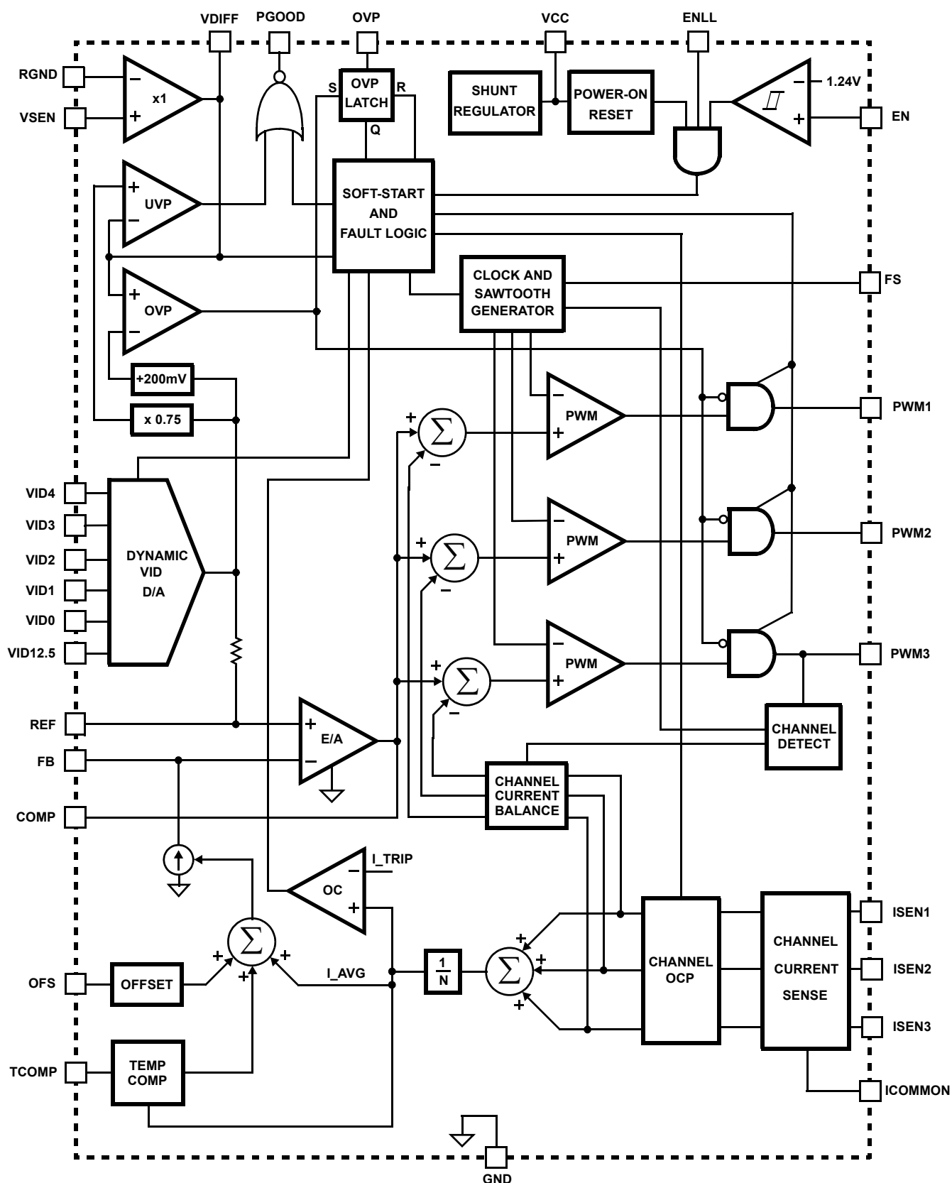
ISL6565B Block Diagram
