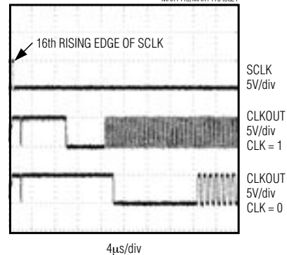
INTERNAL OSCILLATOR STARTUP TIME
