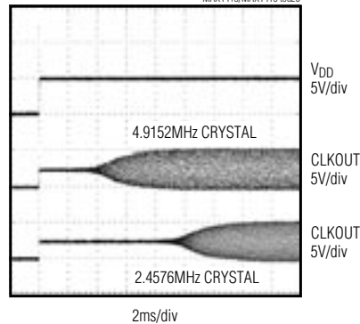
EXTERNAL OSCILLATOR STARTUP TIME
