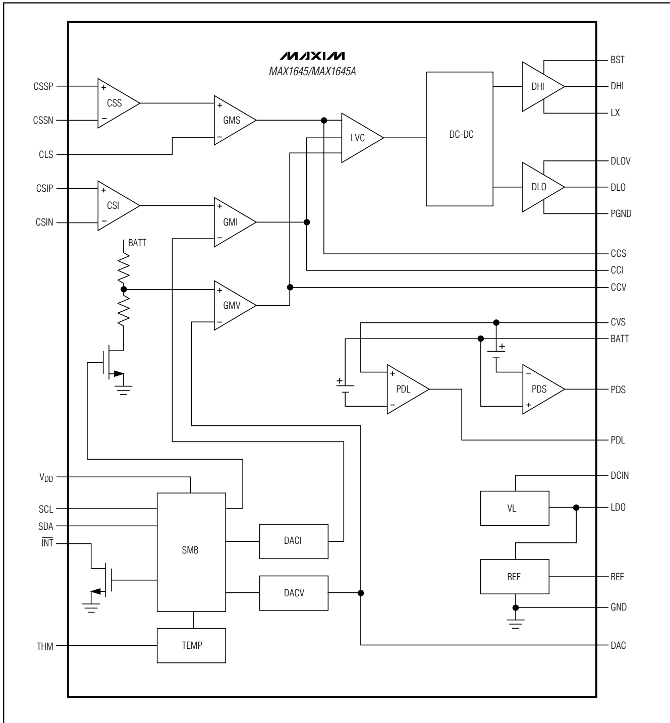
Figure 2. Functional Diagram
