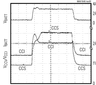
LOAD-TRANSIENT RESPONSE (STEP IN LOAD CURRENT)
