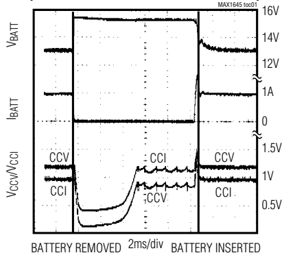
LOAD-TRANSIENT RESPONSE (BATTERY REMOVAL AND REINSERTION)
