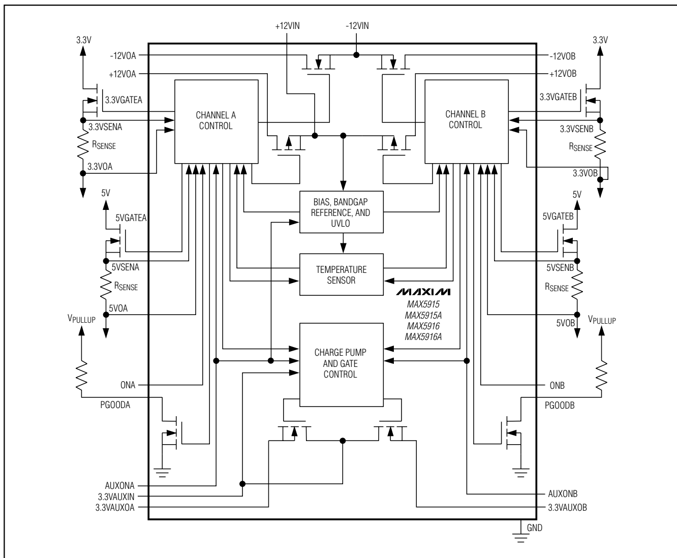
Functional Diagram
