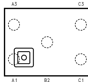
micro SMD, 5 Bump Package (BPA05, TPA05 & BLA05)
