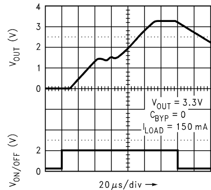
Turn-On Time
