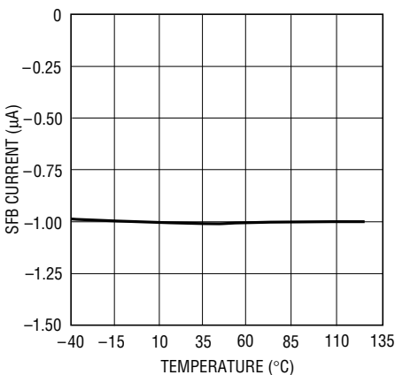
SFB Pin Current vs Temperature
