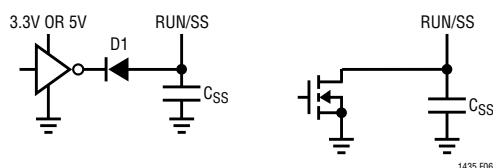
Figure 6. RUN/SS Pin Interfacing
