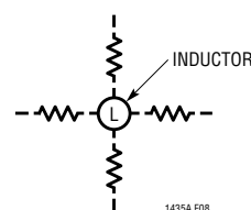
Figure 8. Allowable Inductor/ R_{SENSE} Layout Orientations
