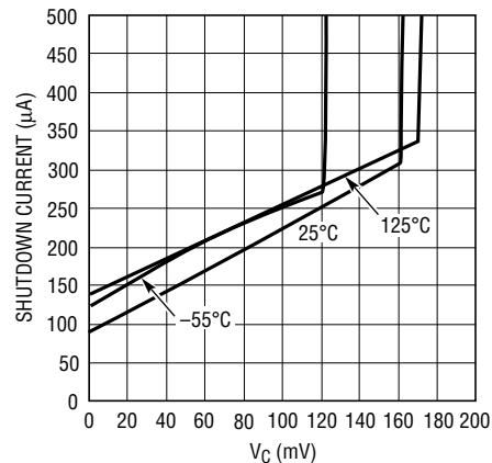
Shutdown Supply Current vs V_C Voltage
