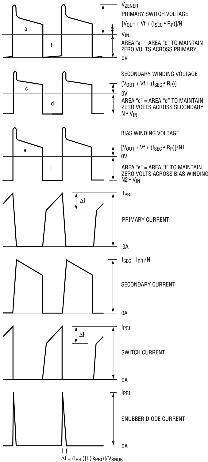
Flyback Waveform for Continuous Mode Operation
