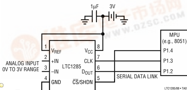
12 \mu W, SO-8 Package, 12-Bit ADC Samples at 200Hz and Runs Off a 3V Supply
