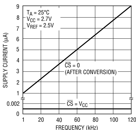
Figure 5. Shutdown Current with \overline{CS} High is 1\text{nA} Typically, Regardless of the Clock. Shutdown Current with \overline{CS} = \text{Ground} Varies From 1\mu\text{A} at 1\text{kHz} to 9\mu\text{A} at 120\text{kHz}
