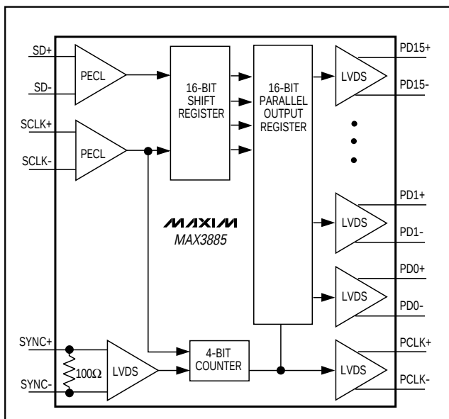
Figure 2. Functional Diagram
