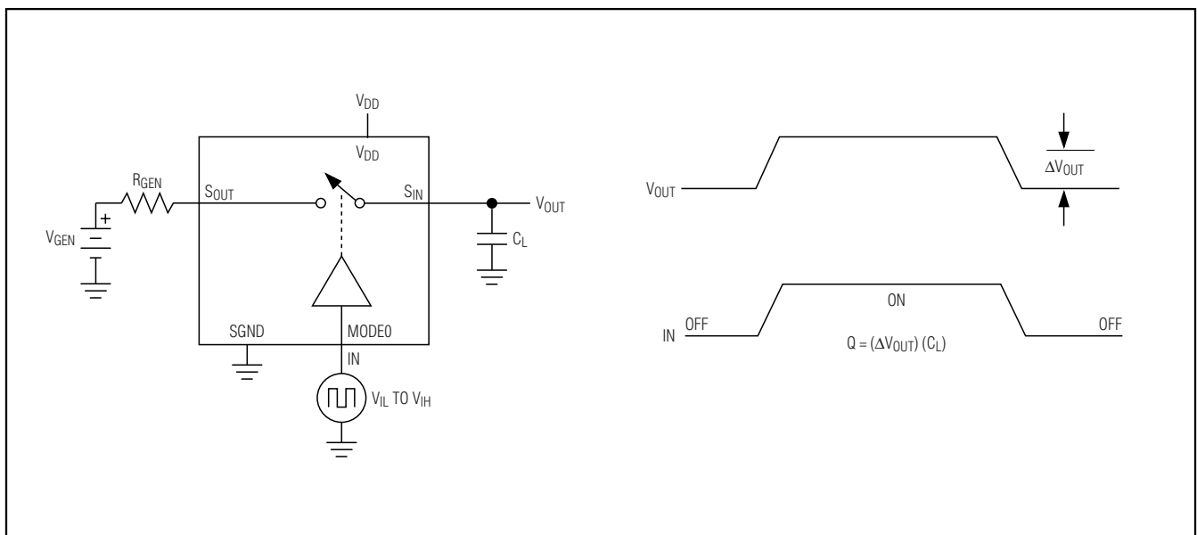
Figure 2. Charge Injection
