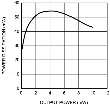
Power Dissipation vs Output Power V_{DD} = 5V, R_L = 32\Omega f = 1kHz, SE, Mode 6
