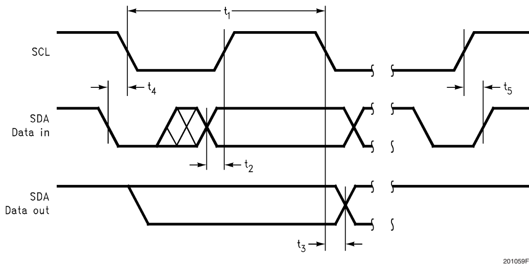
FIGURE 4. I 2 C Timing Diagram
