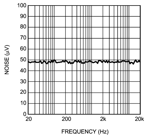
Noise V_{DD} = 3.3V, BTL, Mode 5, BTL
