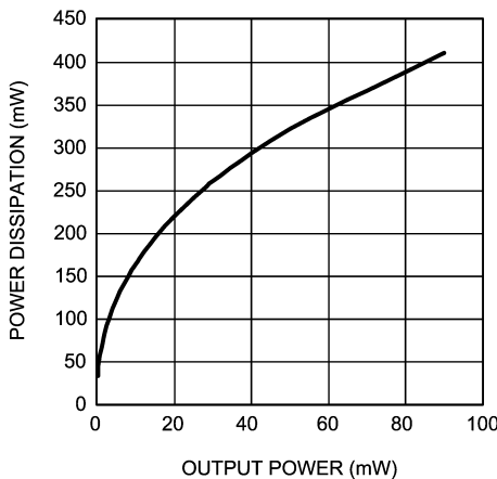
Power Dissipation vs Output Power V_{DD} = 5V , R_L = 32\Omega f = 1kHz , OCL, Mode 6
