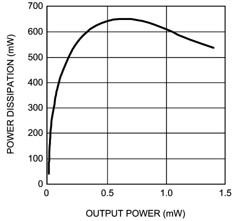
Power Dissipation vs Output Power V_{DD} = 5V , R_L = 8\Omega f = 1kHz , BTL, Mode 1
