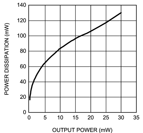
Power Dissipation vs Output Power V_{DD} = 5V , R_L = 32\Omega f = 1kHz , SE, Mode 4
