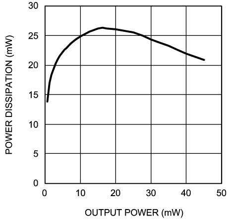
Power Dissipation vs Output Power V_{DD} = 3.3V , R_L = 32\Omega f = 1kHz , SE, Mode 6
