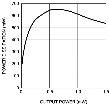
Power Dissipation vs Output Power V_{DD} = 5V , R_L = 8\Omega f = 1kHz , BTL, Mode 5
