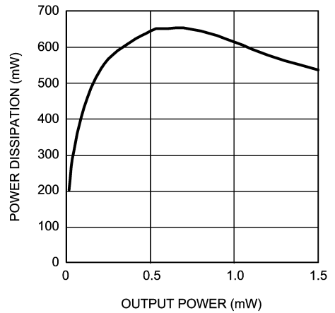
Power Dissipation vs Output Power V_{DD} = 5V , R_L = 32\Omega f = 1kHz , OCL, Mode 4
