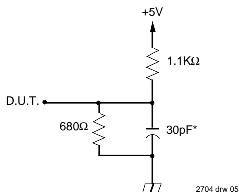
Figure 2. Output Load
