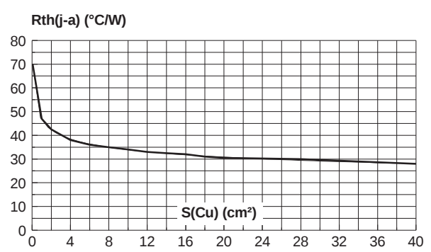
Fig.8 : Thermal resistance junction to ambient versus copper surface under tab (Epoxy printed circuit board FR4, copper thickness : 35 µm). (STPS15L25G only)
