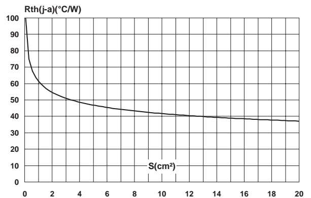
Fig. 10: Thermal resistance junction to ambient versus copper surface under tab (epoxy printed board FR4, \text{Cu} = 35\mu\text{m} ).
