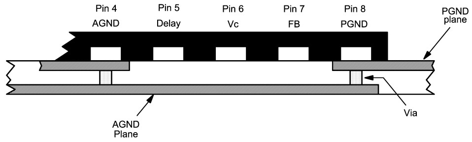
FIGURE 3. Multi-Layer Layout
