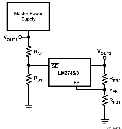
FIGURE 6. Sequencing Circuit
