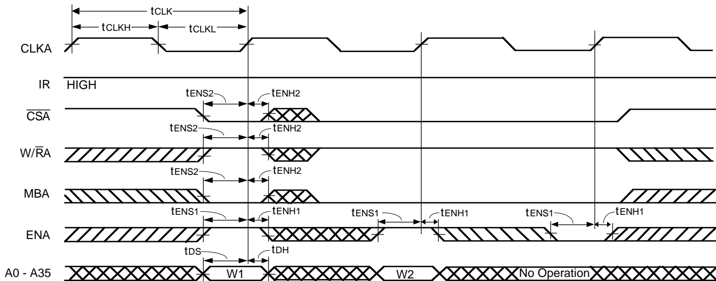
Figure 4. FIFO Write-Cycle Timing
