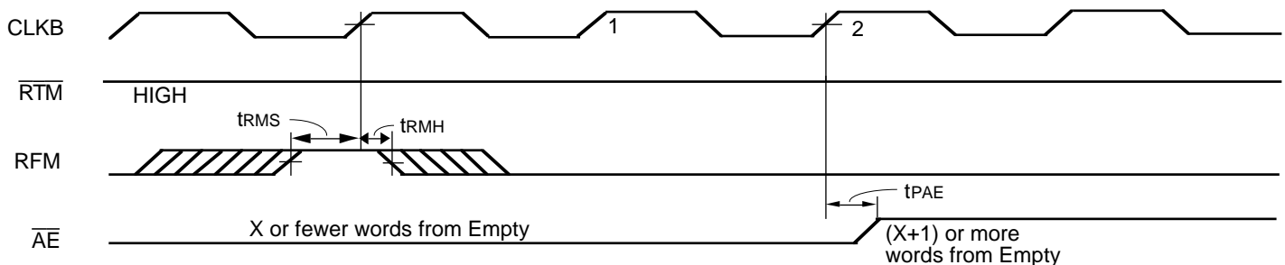
Figure 11. \overline{AE} Maximum Latency When Retransmit Increases the Number of Stored Words Above X.
