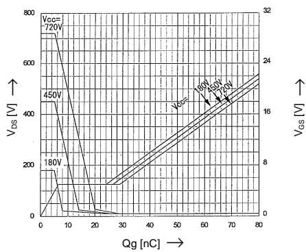
Typical Gate Charge Characteristics V_{GS} = f(Q_g) ; I_D = 5\text{A}
