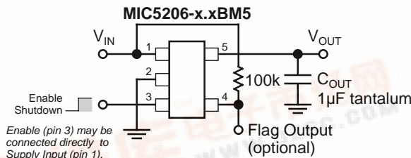
SOT-23-5 Fixed Voltage Application
