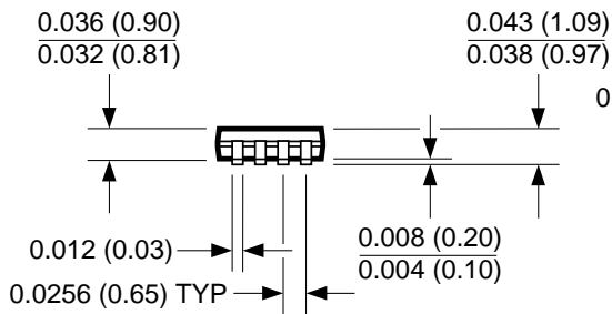
8-Lead MSOP (MM)
