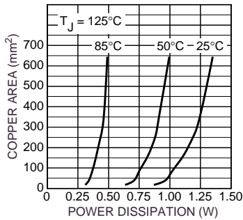
Figure 7. Copper Area vs. Power-SOP Power Dissipation ( T_A )
