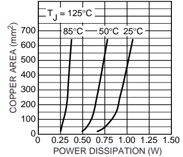
Figure 9. Copper Area vs. Power-MSOP Power Dissipation ( T_A )
