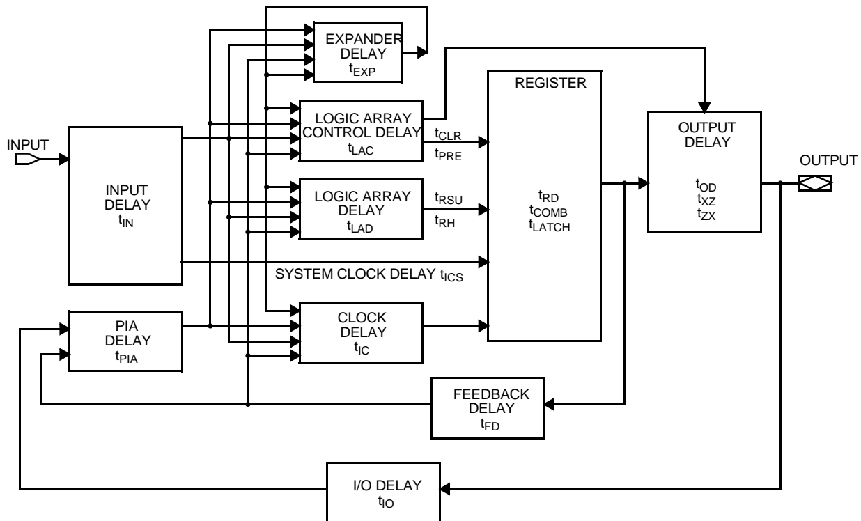
Figure 1. CY7C346 Internal Timing Model
