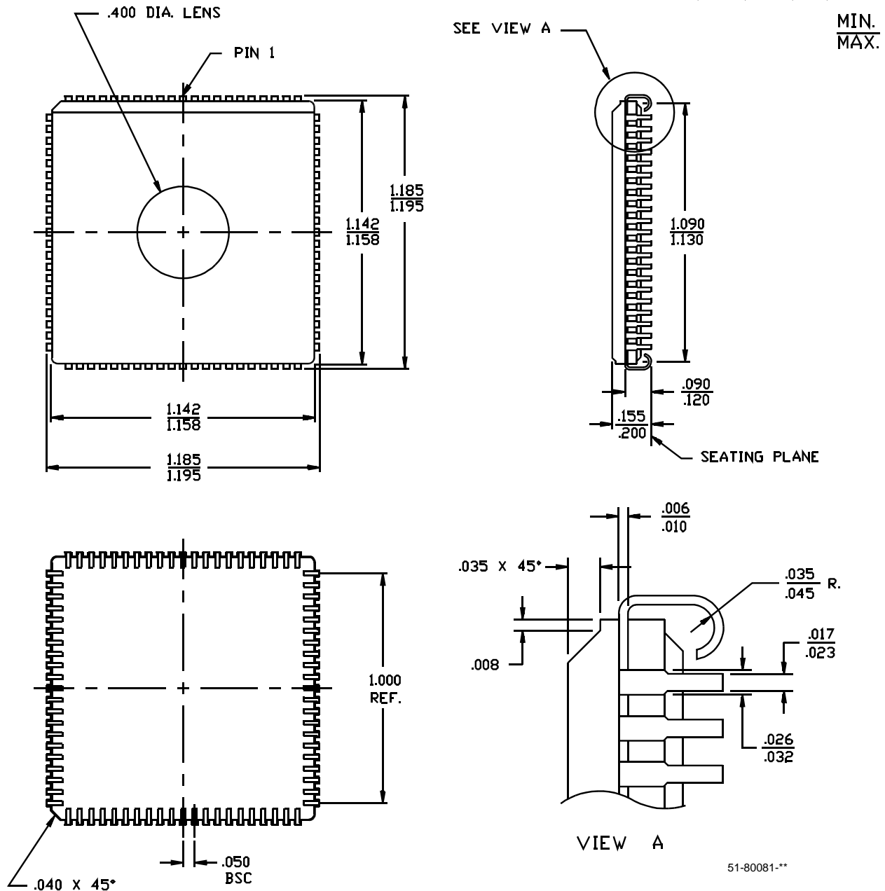
84-Leaded Windowed Leaded Chip Carrier H84
