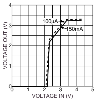
Dropout Characteristics
