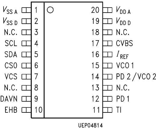
P-DSO-20-1
