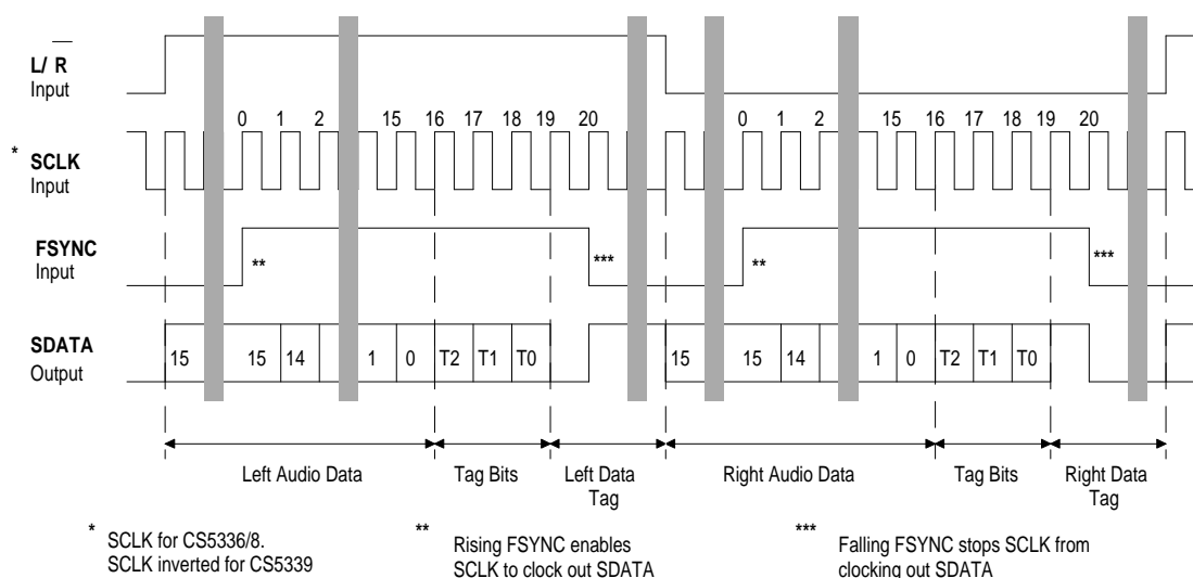
Figure 5. Data Output Timing - SLAVE Mode, FSYNC controlled
