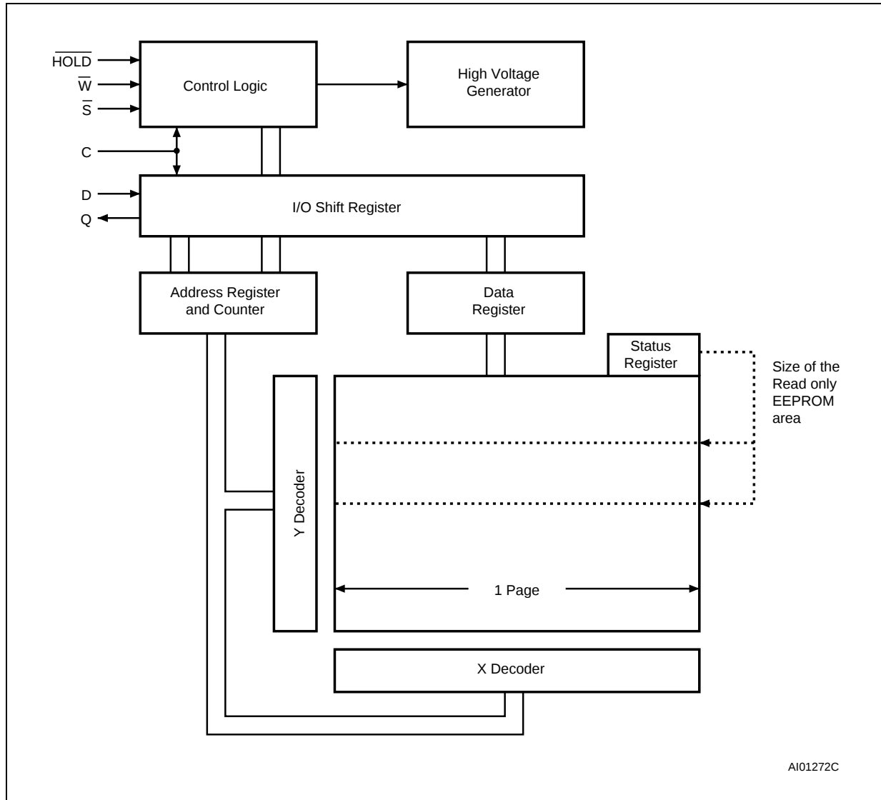
Figure 7. Block Diagram
