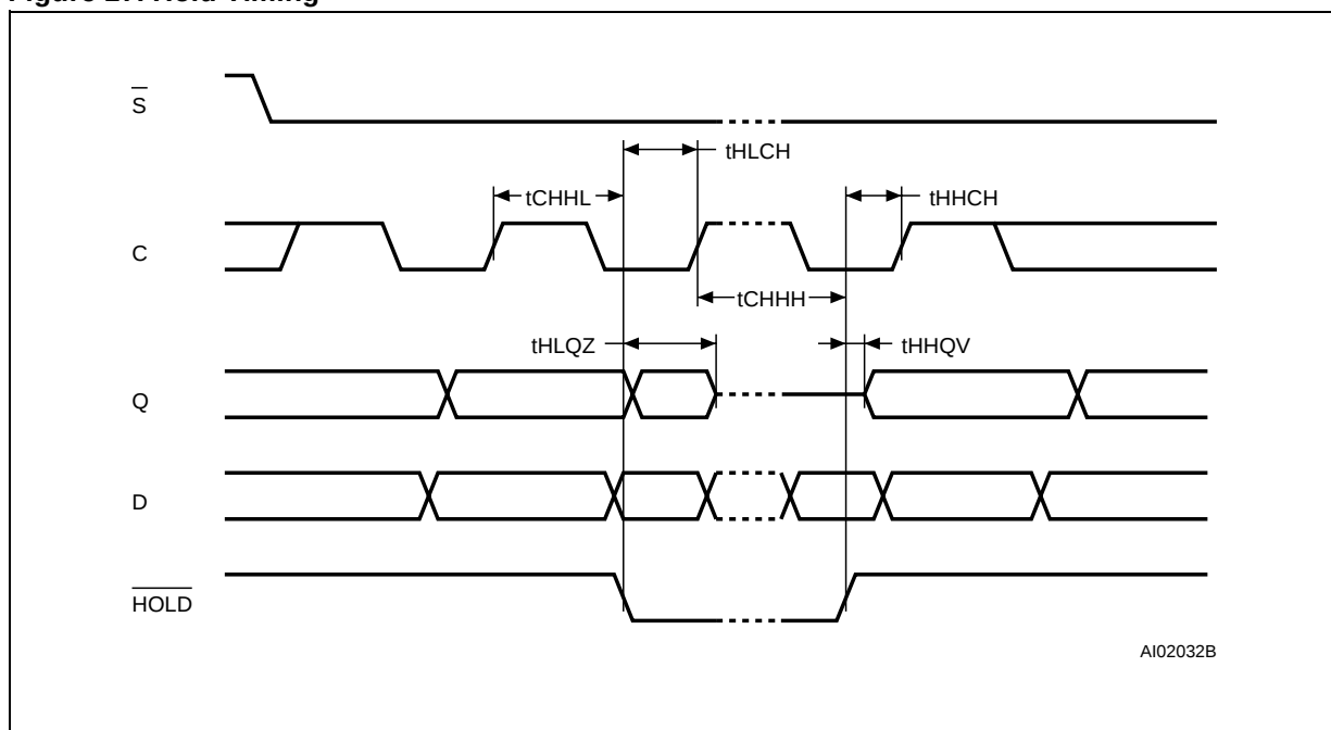
Figure 17. Hold Timing
