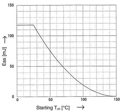
Avalanche Energy Derating E_{as} = f(\text{starting } T_{ch}) ; V_{CC} = 60\text{V} ; I_{AV} = 9\text{A}
