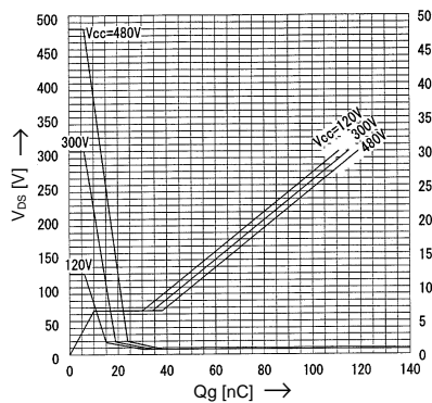
Typical Gate Charge Characteristic V_{GS} = f(Q_g) ; I_D = 9\text{A} ; T_{ch} = 25^\circ\text{C}
