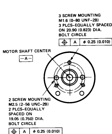
Figure 2. Mounting Holes.
