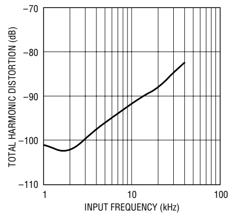
Total Harmonic Distortion vs Input Frequency (LTC1605-2)
