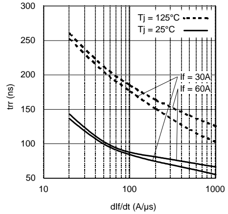
Fig. 8 - Typical Reverse Recovery Time vs. di/dt
