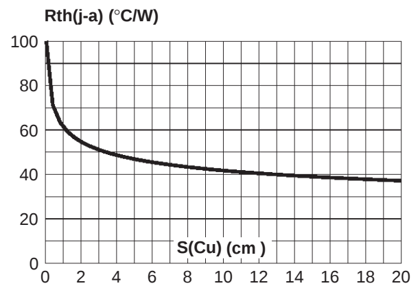
Fig. 8: Thermal resistance junction to ambient versus copper surface under tab (Epoxy printed circuit board FR4, copper thickness: 35μm).
