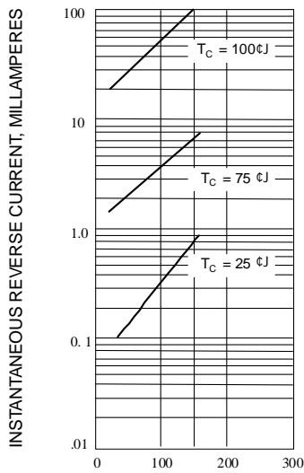
Fig. 3-TYPICAL REVERSE CHARACTERISTICS
