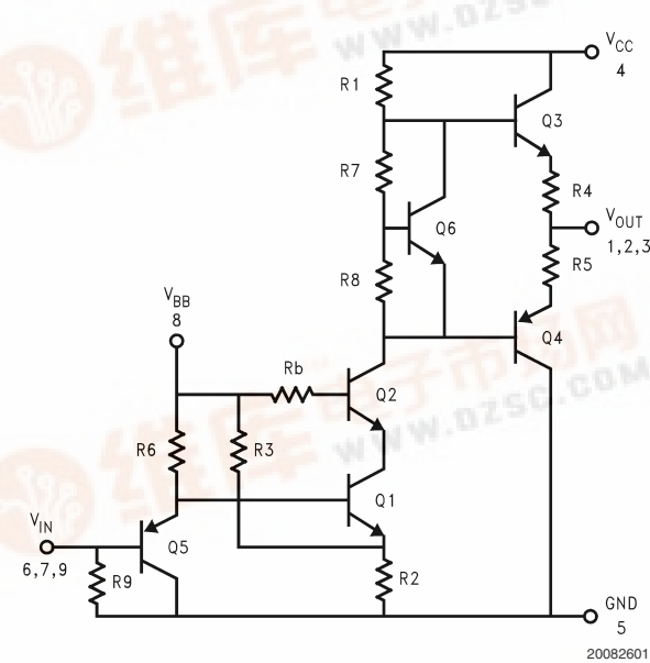
FIGURE 1. Simplified Schematic Diagram (One Channel)
