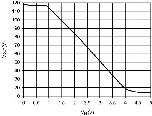
FIGURE 3. V IN vs V OUT
