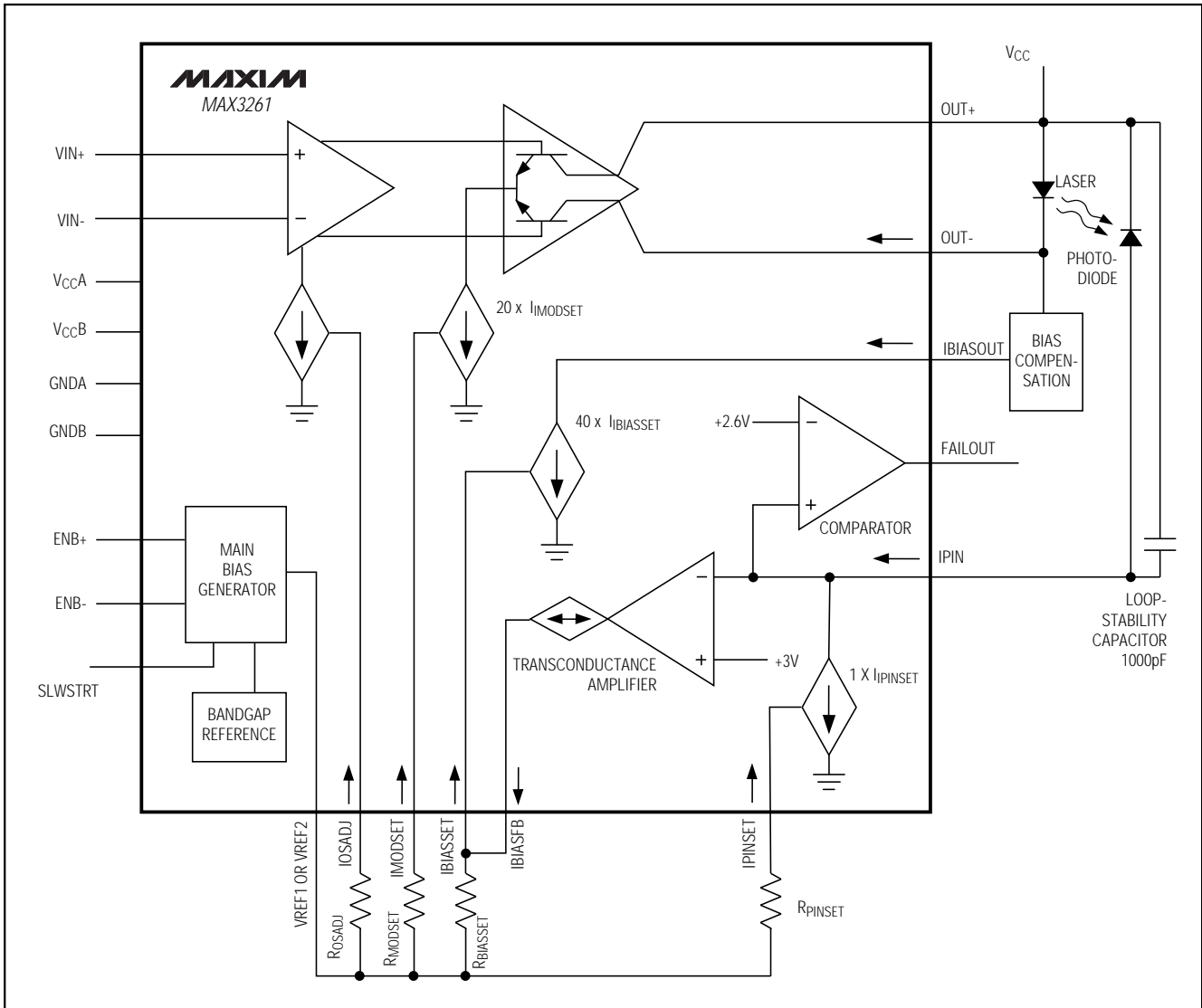
Figure 1. Functional Diagram
