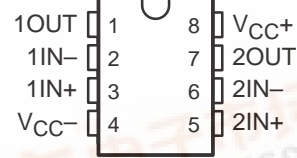
TLV2362 . . . D, P, OR PW PACKAGE (TOP VIEW)
