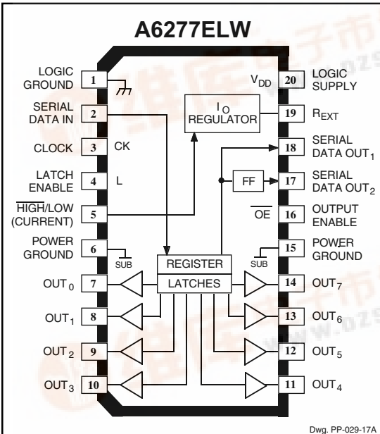
Dwg. PP-029-17A
