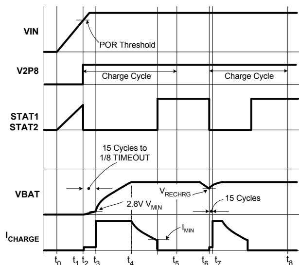
FIGURE 4. OPERATION WAVEFORMS
