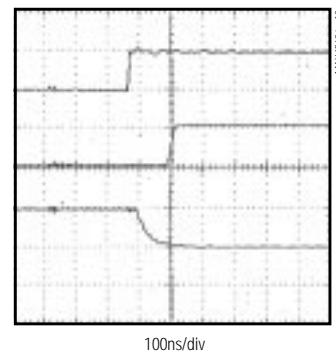
TURN-ON AND TURN-OFF TIMES (HARD MODE)
