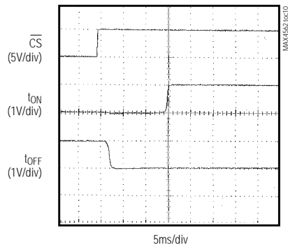
TURN-ON AND TURN-OFF TIMES (SOFT MODE)
