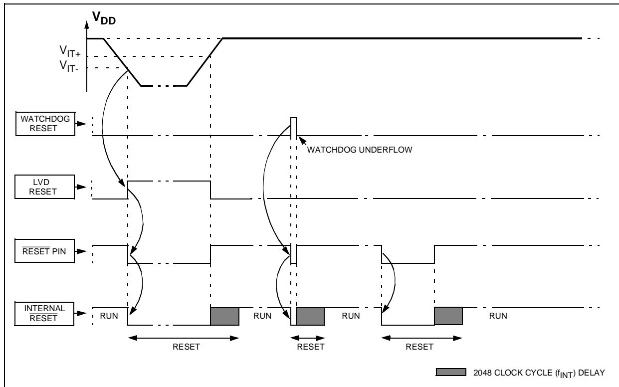
Figure 13. RESET Sequence
