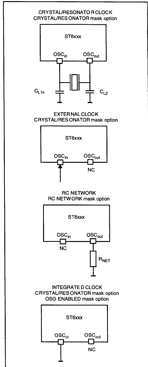
Figure 11. Oscillator Configurations
