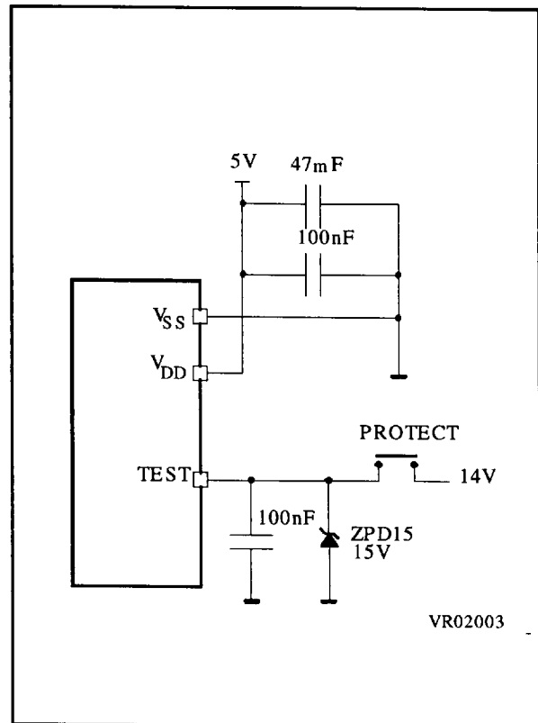
Figure 34. Programming Circuit
