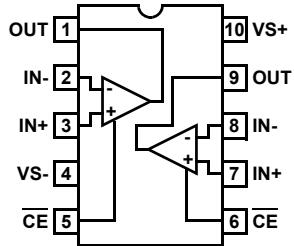
EL5262 (10-PIN MSOP) TOP VIEW
