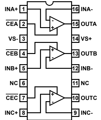
EL5362 (16-PIN SO (0.150"), QSOP) TOP VIEW
