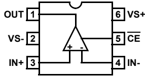
EL5162 (6-PIN SOT-23) TOP VIEW
