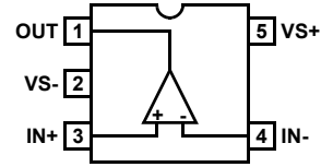
EL5163 (5-PIN SOT-23, SC-70) TOP VIEW
