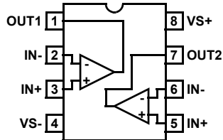
EL5263 (8-PIN SO, MSOP) TOP VIEW
