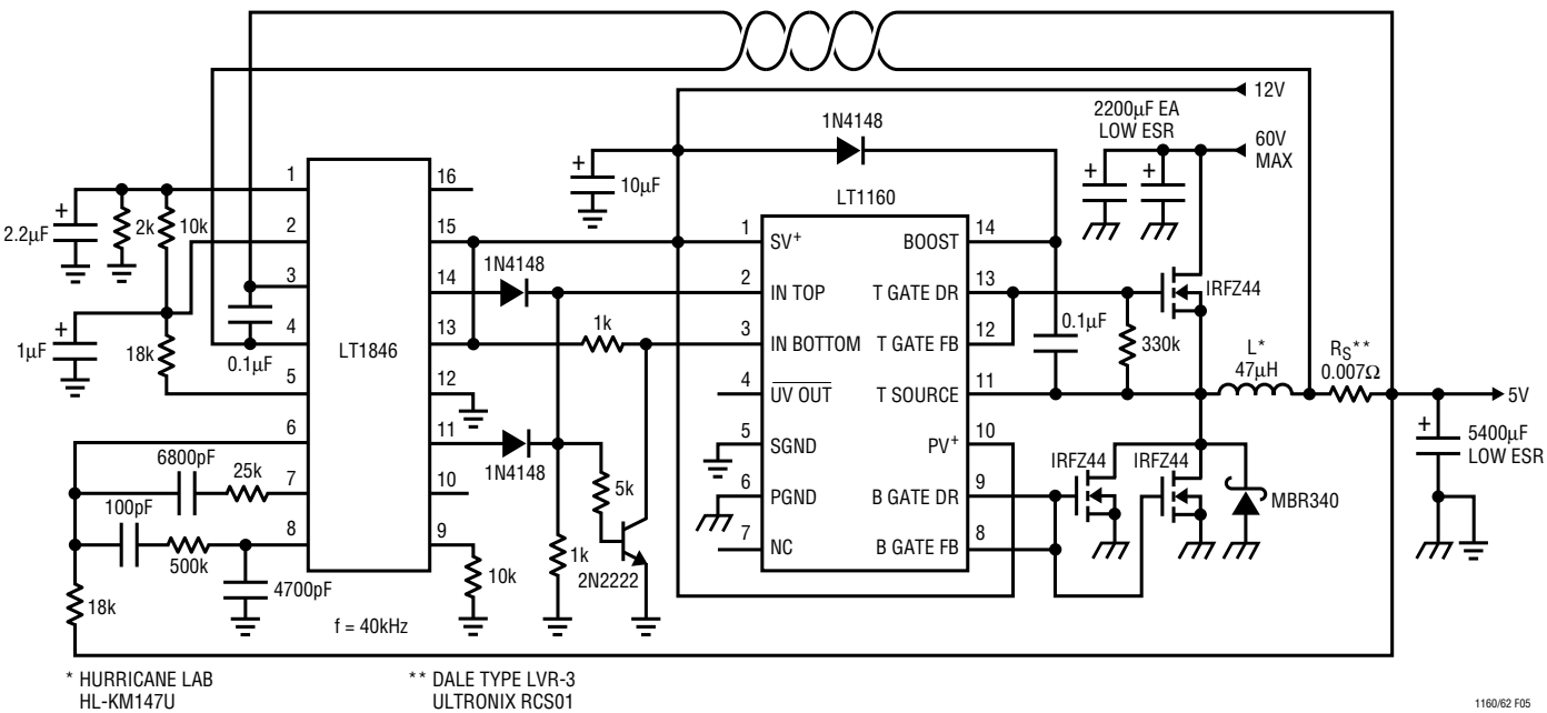
Figure 5. 90% Efficiency, 40V to 5V 10A Low Dropout Current Mode Switching Regulator
