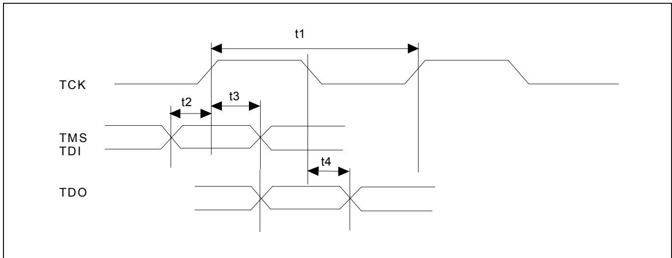
Figure 9-14. JTAG Timing
