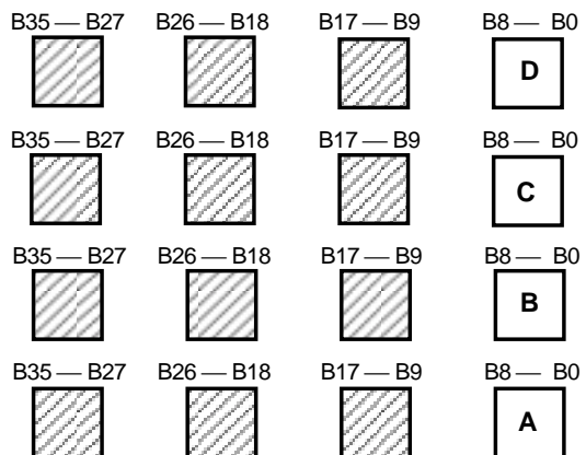
Figure 2. Bus sizing
