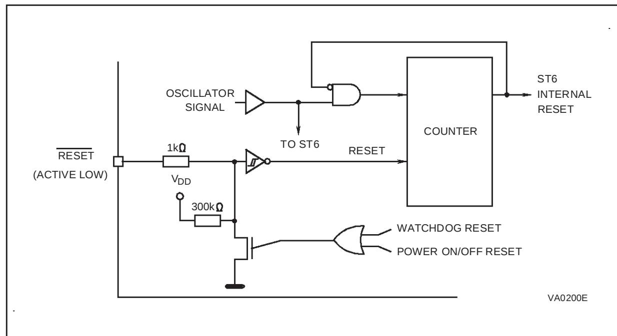
Figure 15. Reset Circuit
