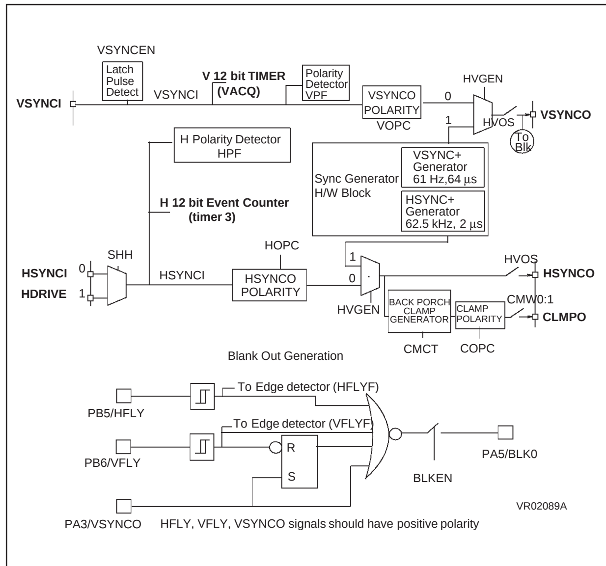
Figure 27. SYNC Processor Block Diagram
