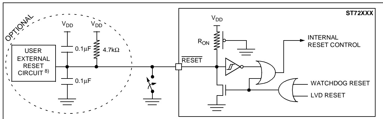
Figure 72. Typical Application with RESET pin 7)
