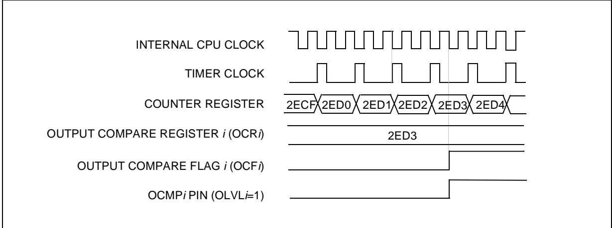
Figure 31. Output Compare Timing Diagram, f_{\text{TIMER}} = f_{\text{CPU}}/2
