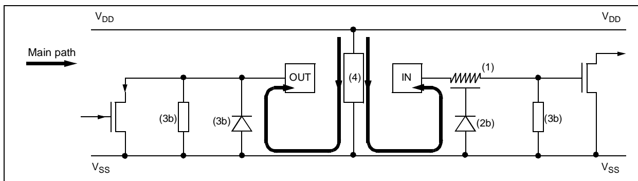
Figure 60. Multisupply Configuration
