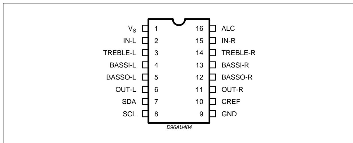
Figure 3. Pin Connection
